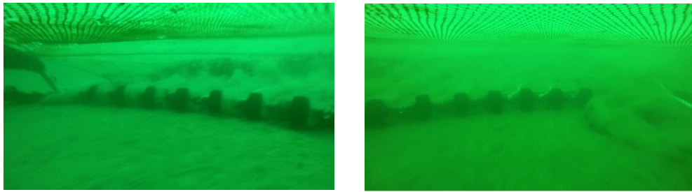
Figure 4: Left: Strong resuspension of sediment by lateral rolls. Right: Strong sediment turbulence caused by the middle chain of the bridle.
